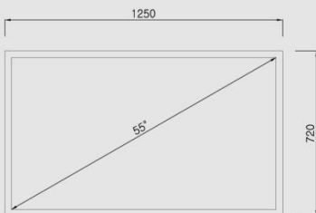
▲ FORNT VIEW
